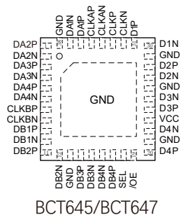
QFN4x4-38L
