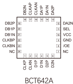
QFN3.4x2.5-24L
