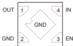
UTDFN1x1-4L DFN1x1-4L
