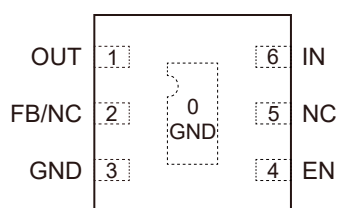
DFN2x2-6L
