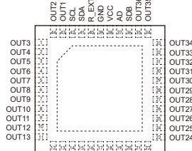
QFN5x5-44L
