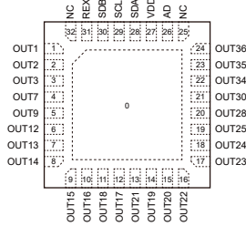
BCT3024X
