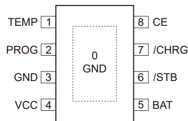
BCT4056
