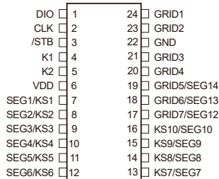
BCT3668X/BCT1668X
