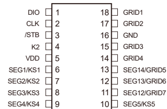
BCT3618
