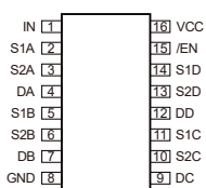
BCT4330
