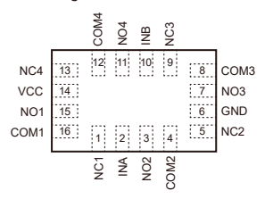
BCT4699/BCT4899
