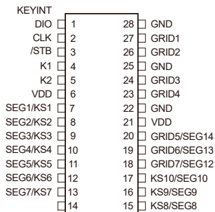
BCT3627
