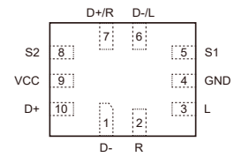
BCT4321N
