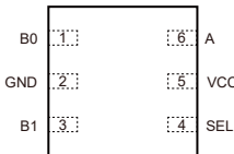
BCT4157
