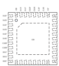
QFN4x4-38L
