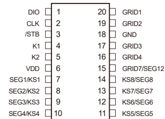
BCT3622
