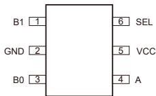
BCT4157
