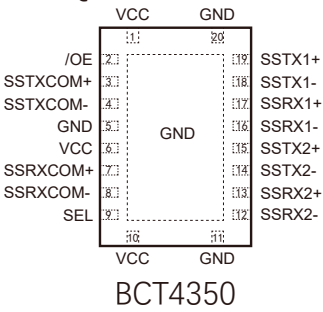
TQFN4.5x2.5-20L
