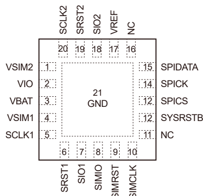
BCT4302B
