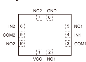
QFN1.8x1.4-10L
