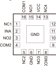
BCT4699/BCT4899
