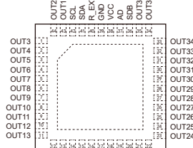
QFN5x5-44L
