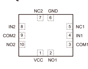
BCT4717A
