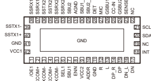
BCT4888
