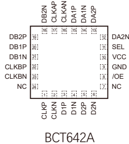
QFN3.4x2.5-24L
