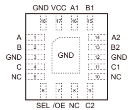
QFN2.8x2.0-18L
