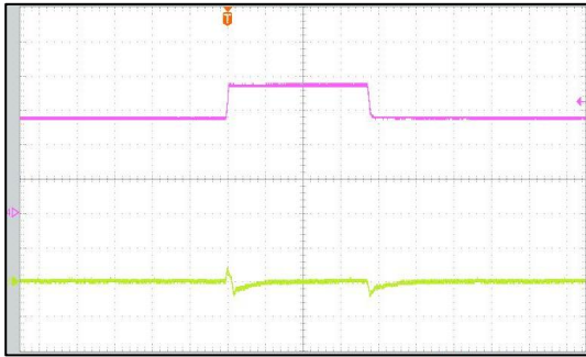
Load Transient Response ( V_{OUT}=1.8V )
